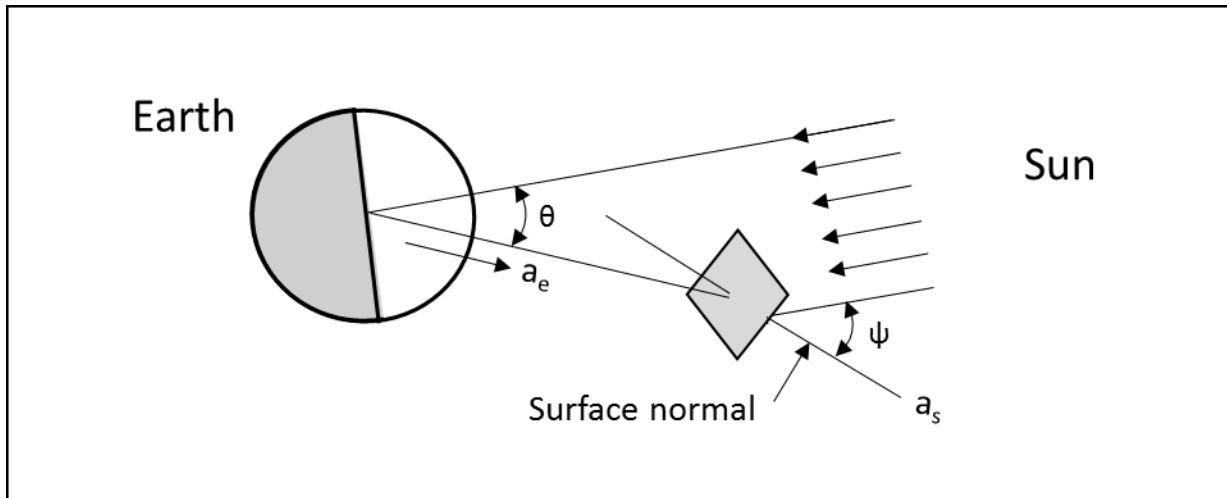
Figure 12. Orbital Heating Sources and Geometry
