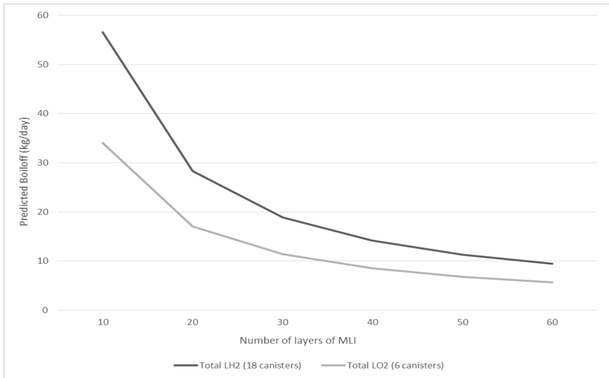
Figure 16. Boiloff Rates for CSSV Canister Fuel Tanks in LEO.
